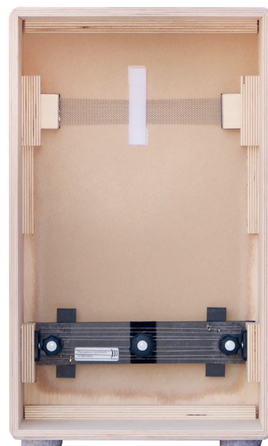
Picutre shows details of CP580
